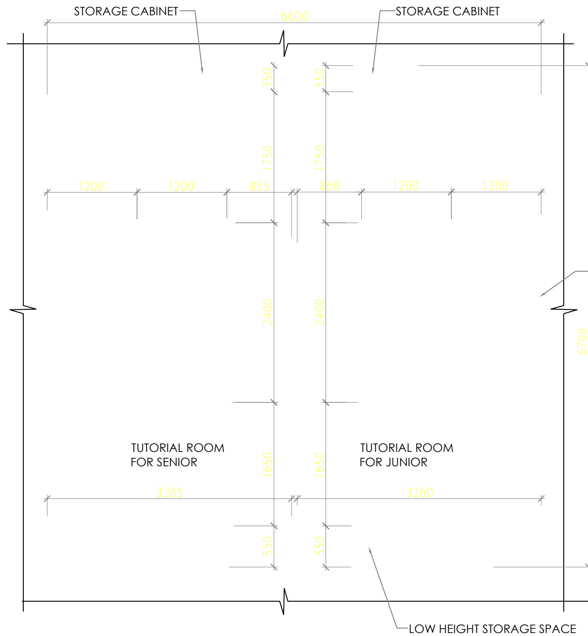
TUTORIAL (CAPACITY - 30 ) SCALE - 1:50
